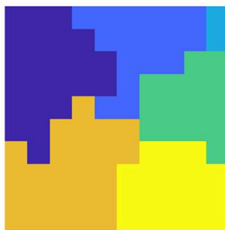
Figure 12. Segmentation of texture regions that are images of surfaces slanted in depth. This demonstrates the effectiveness and importance of transitive grouping. Note the segmentation error in the upper right corner of example B. This failure occurred because region grouping failed (the patches in the small region are not very similar to any of those in the large region). If the texture regions are correctly segmented, then the systematic changes in the texture can be used to estimate 3D geometry.
